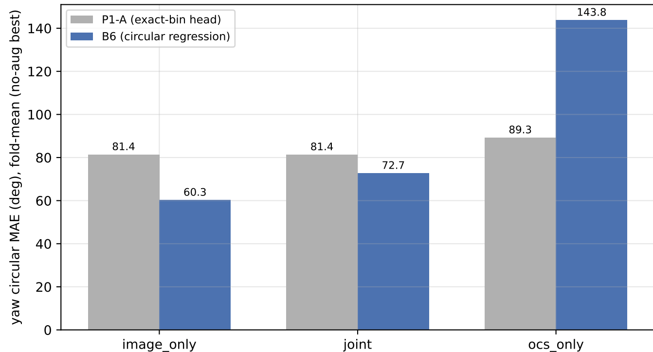
SI-1 B6 single-frame / yaw-block closure: circular regression improves image/joint cMAE but yaw extrapolation still fails
