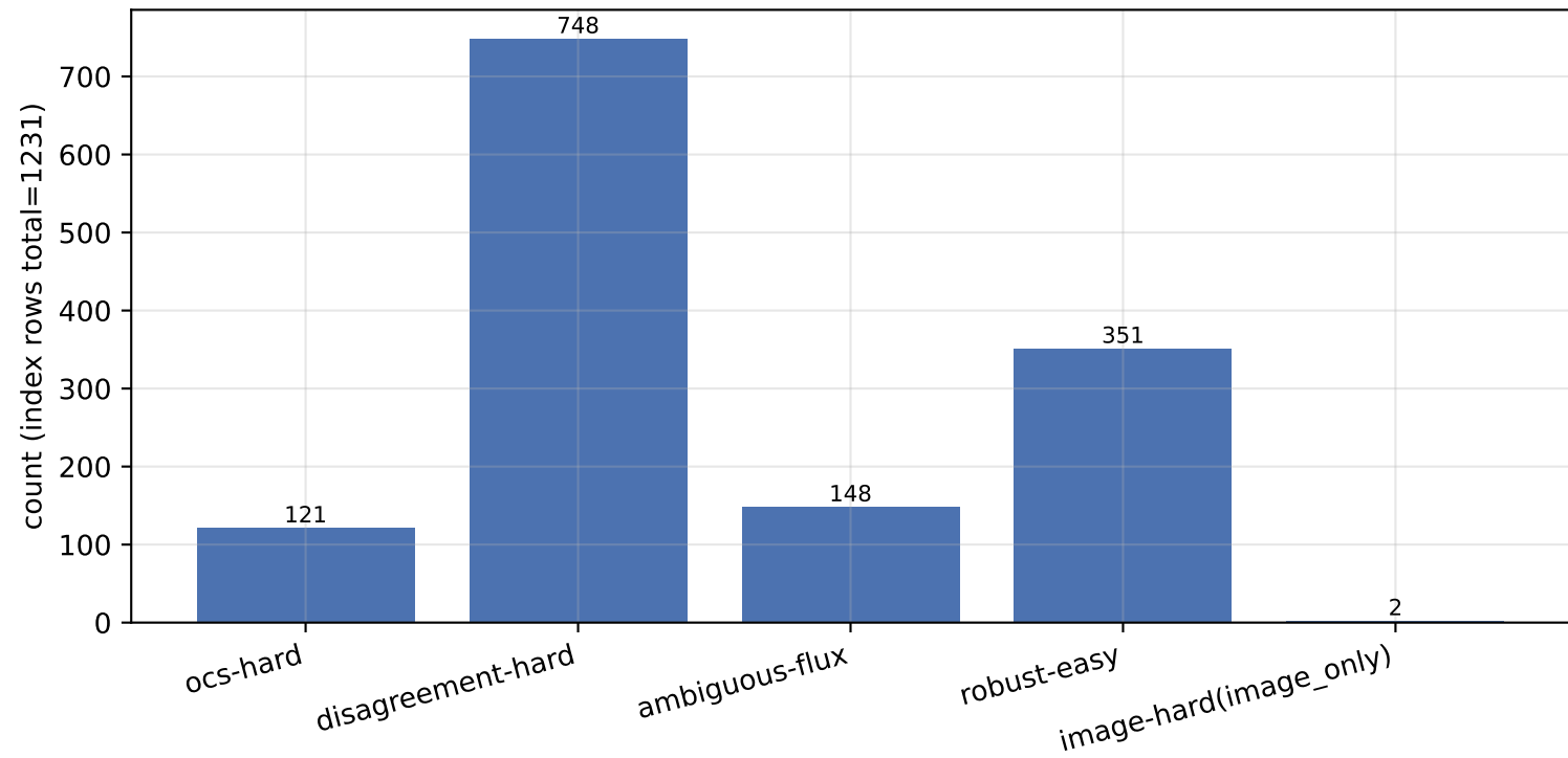
SI-4 hard-case index label distribution (candidate input for future P-INT-hard; NOT a stage-gate release)
