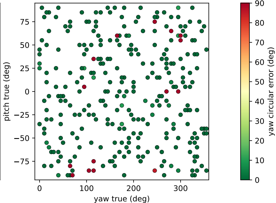
P-DB G5 yaw err (neg-L2 matched)
