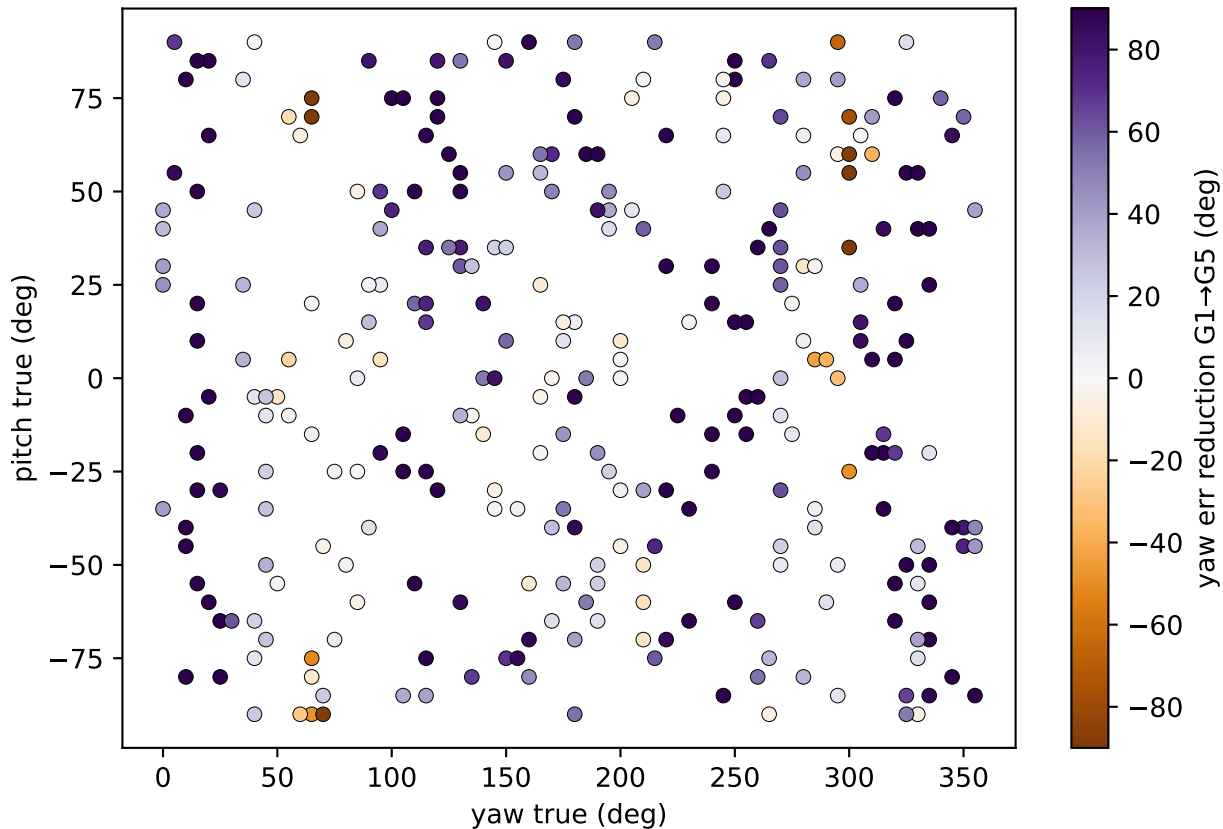
D4 geometry gain map: OCS-only (G1 err – G5 err), positive=G5 rescues — simulated
