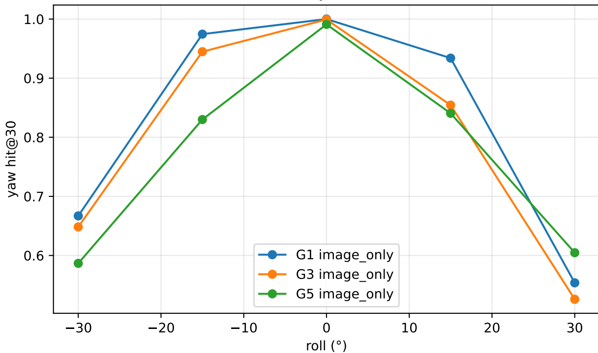
M-roll full-2664: yaw hit@30 vs roll
