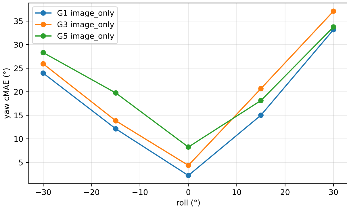
M-roll full-2664: yaw cMAE vs roll
