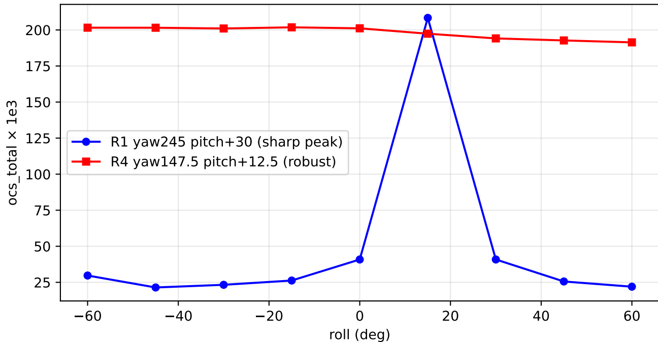
R1 vs R4 roll curve comparison (phase63/L1-G1)
