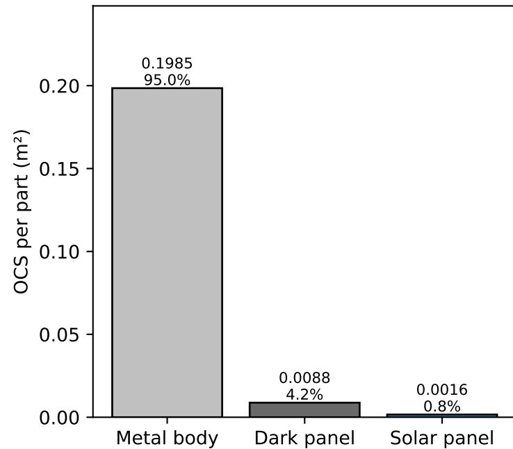
top-1 OCS per-part yaw245/pitch27.5/roll+15
