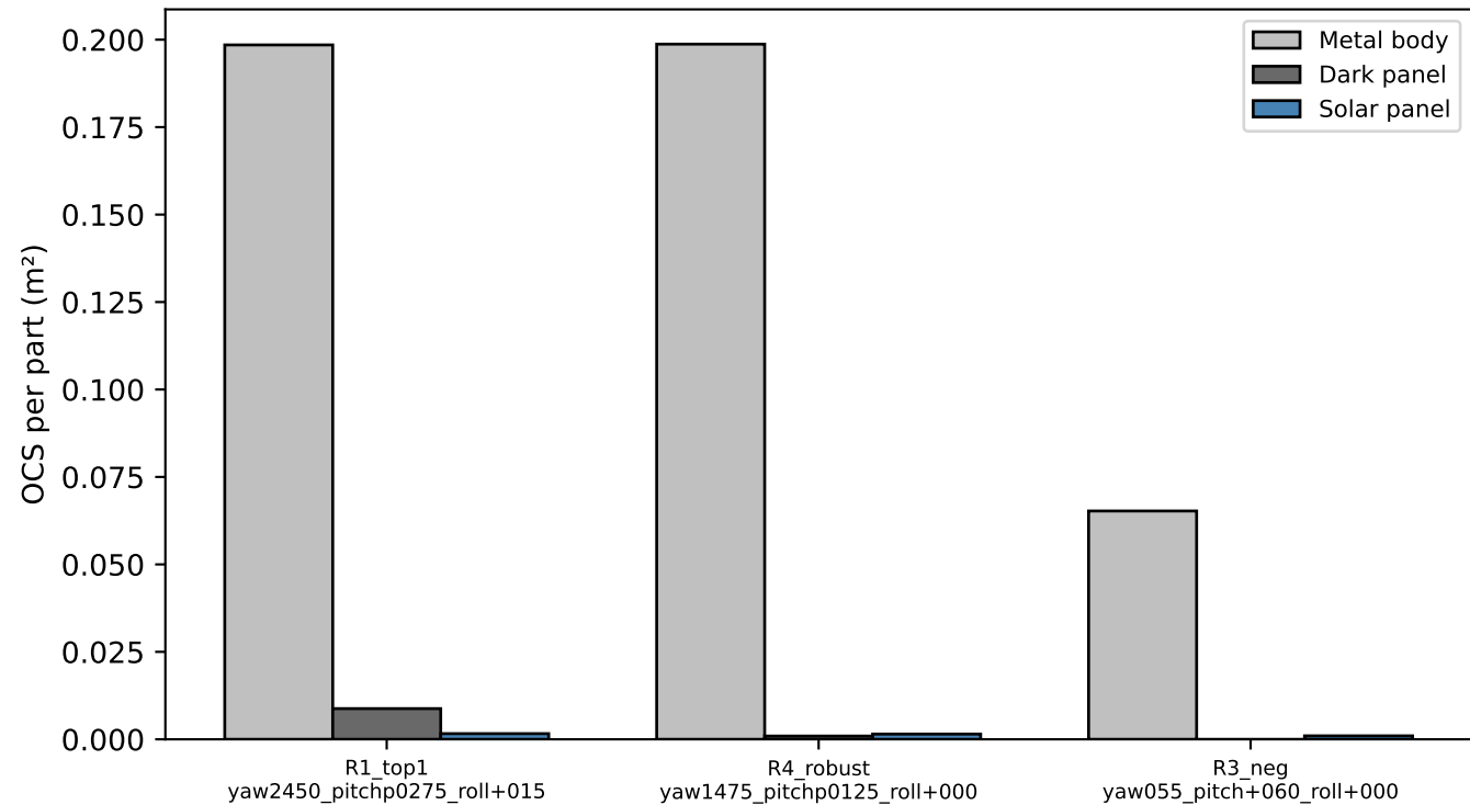
top-1 vs R4 vs R3 per-part OCS contribution
