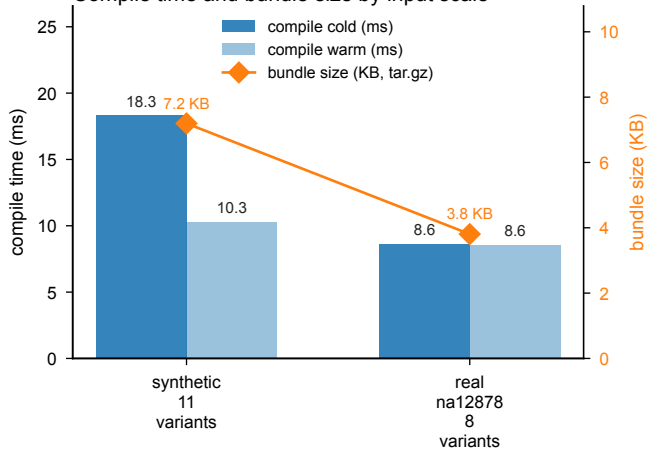
a Compile time and bundle size by input scale
