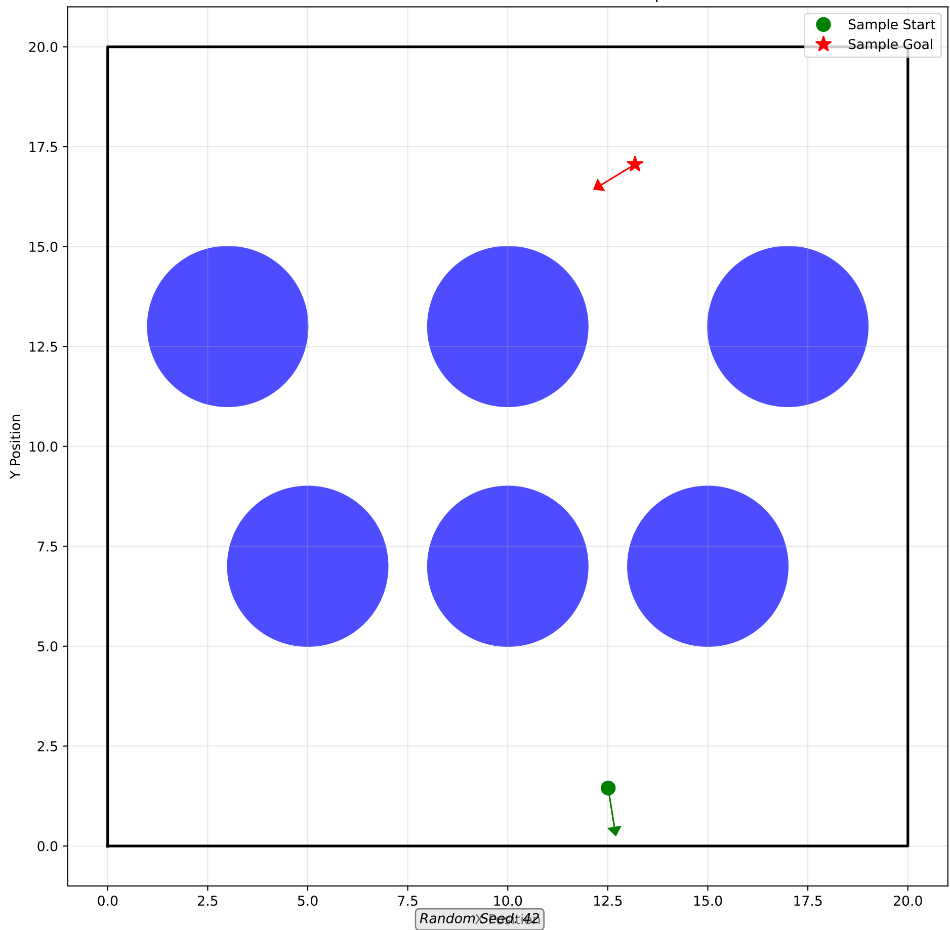
Obstacle Environment for RRT vs RRT* Comparison
