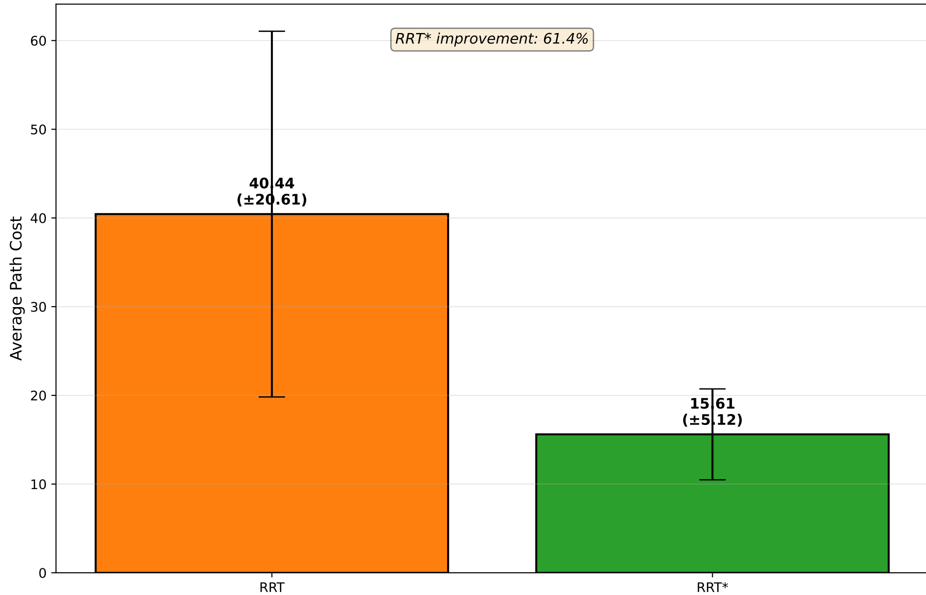
RRT vs RRT* Average Path Cost Comparison (100 Random Instances)
