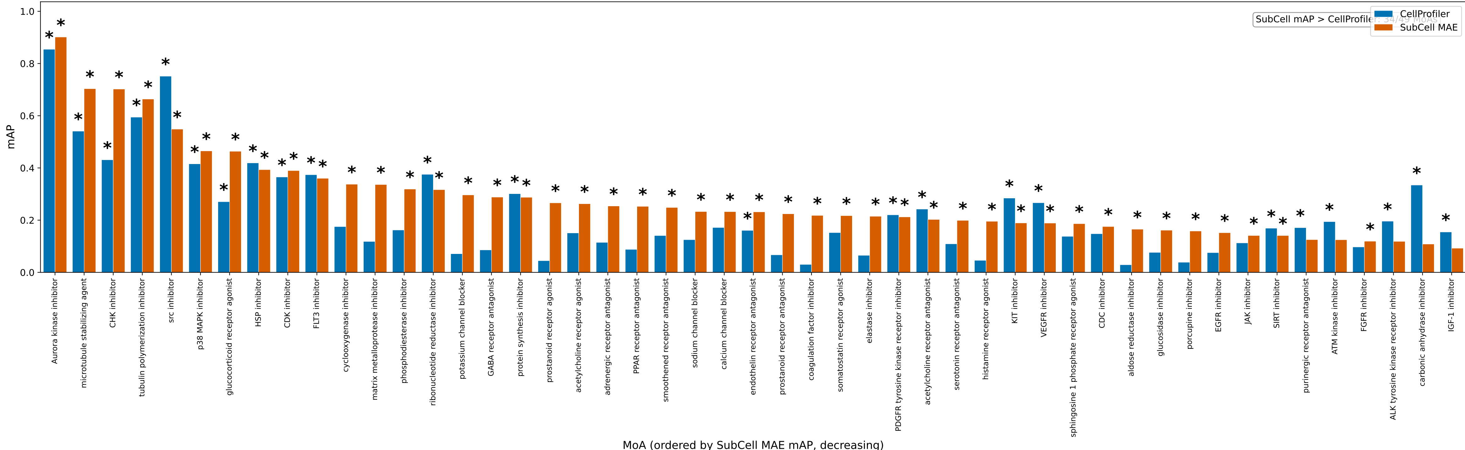
U2OS — Per-MoA mAP (* = corrected p < 0.05)
