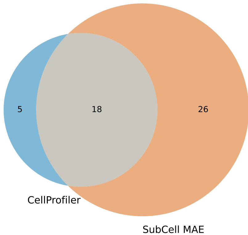
U2OS — Significantly Retrieved MoAs (corrected p < 0.05 )
