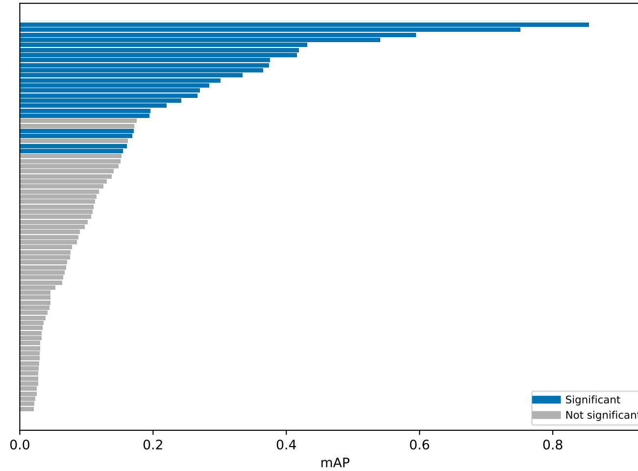
CellProfiler (23/77 significant)
