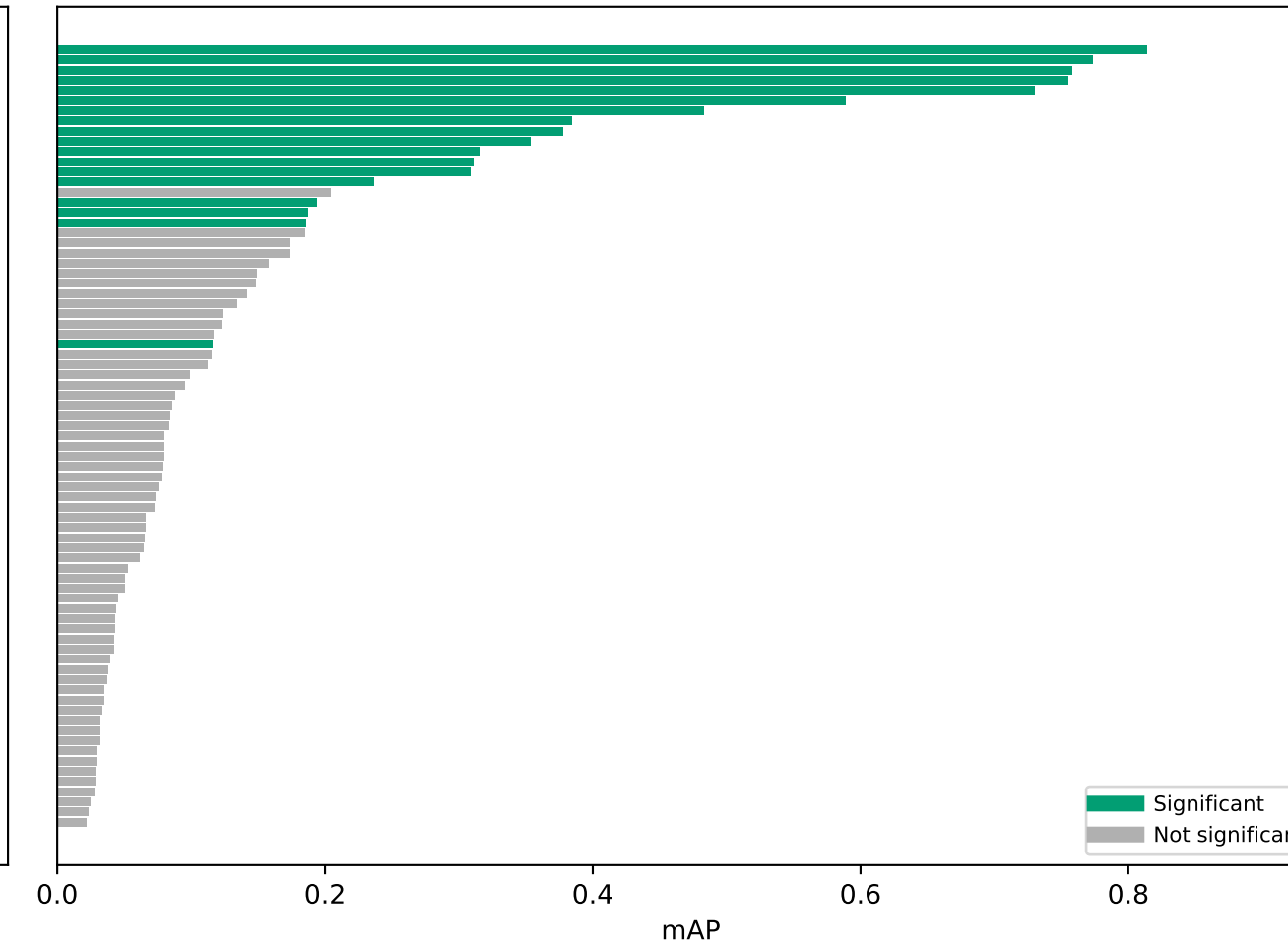
DINO4Cells (18/77 significant)
