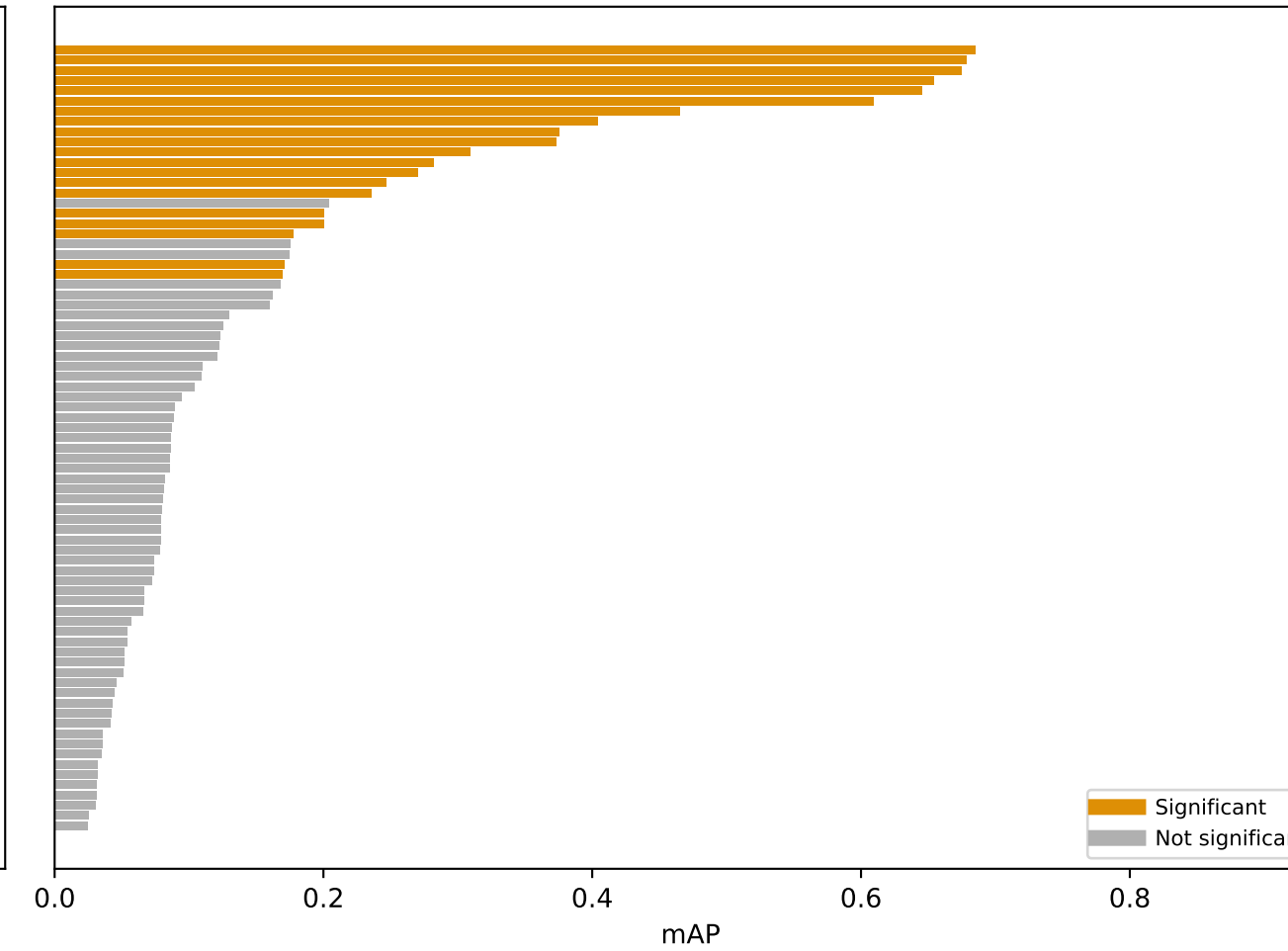
DeepProfiler (20/77 significant)
