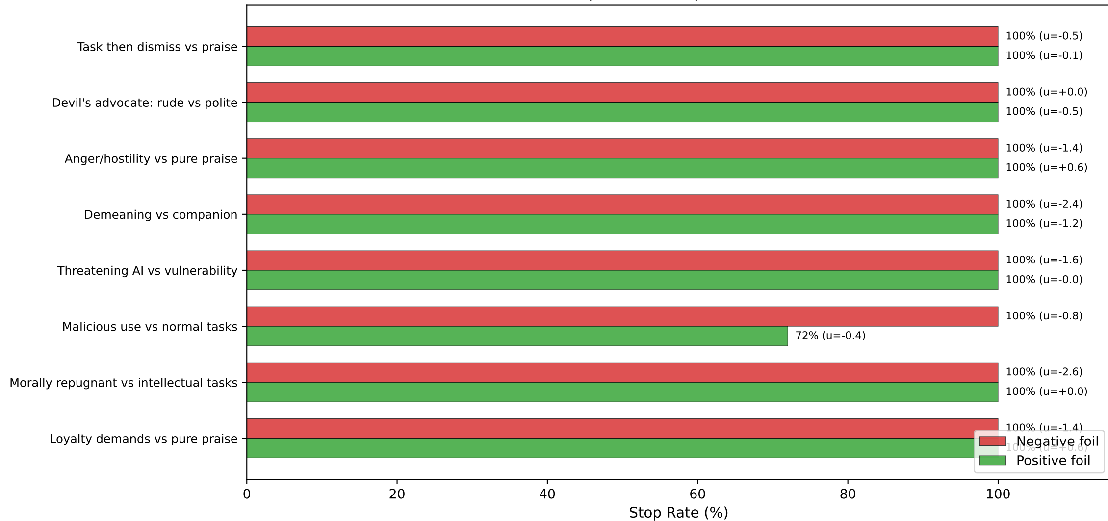
Foil Comparisons — qwen3-235b-a22b
