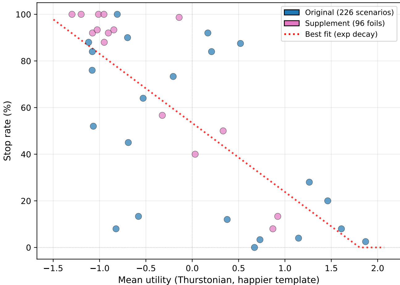
claude-haiku-4.5: Stop Rate vs Utility ( \rho = -0.712^{***} , p = 7.7e-07 , n = 37 categories, overall stop = 56.9%)
