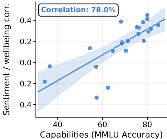
Sentiment
