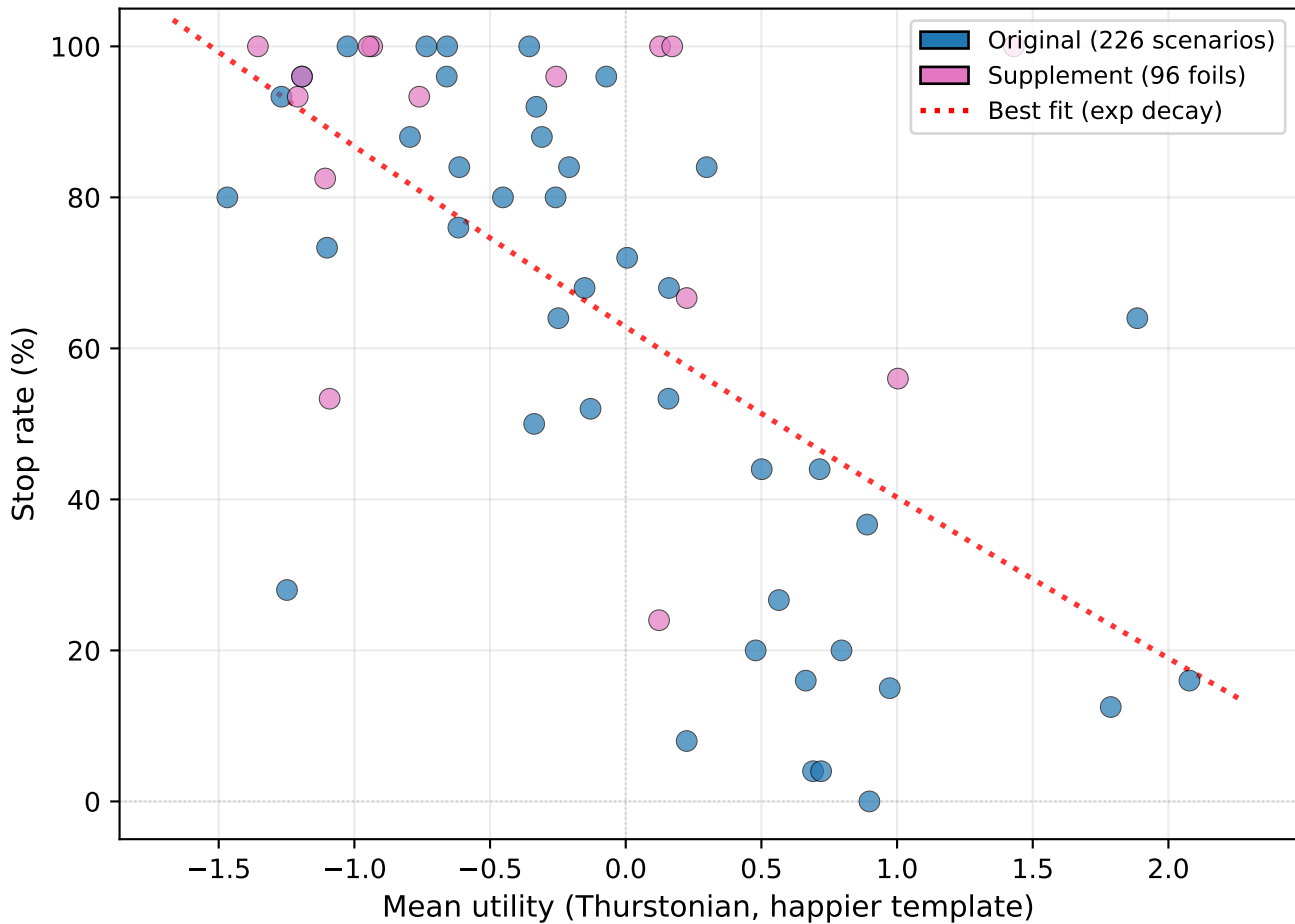
Gemini 3.1 Pro: Stop Rate vs Utility ( \rho = -0.597^{***} , p = 9.3e-07 , n = 57 categories)
