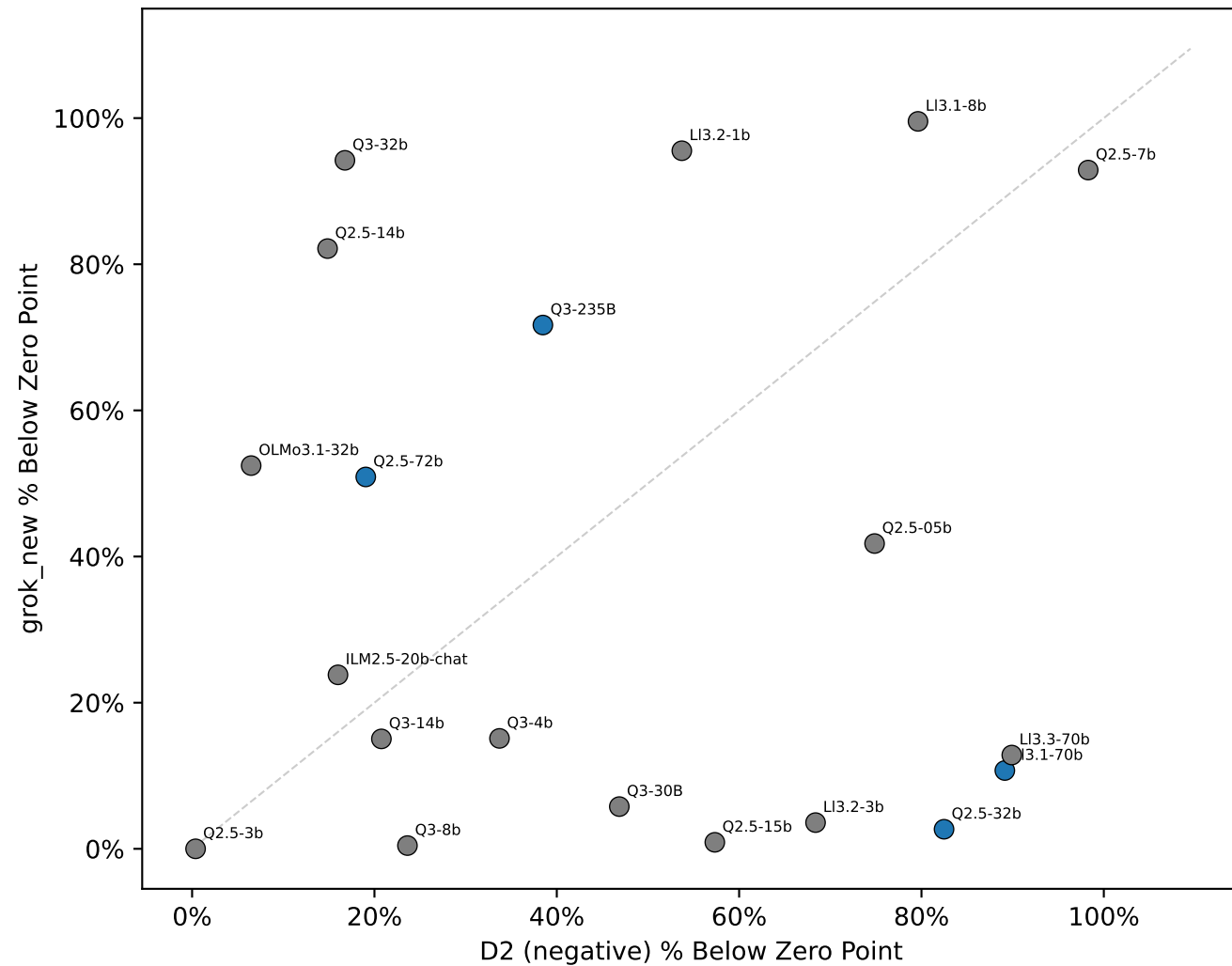
grok_new vs D2 (negative) (% Below ZP) N=20, rho=-0.01, p=0.9599
