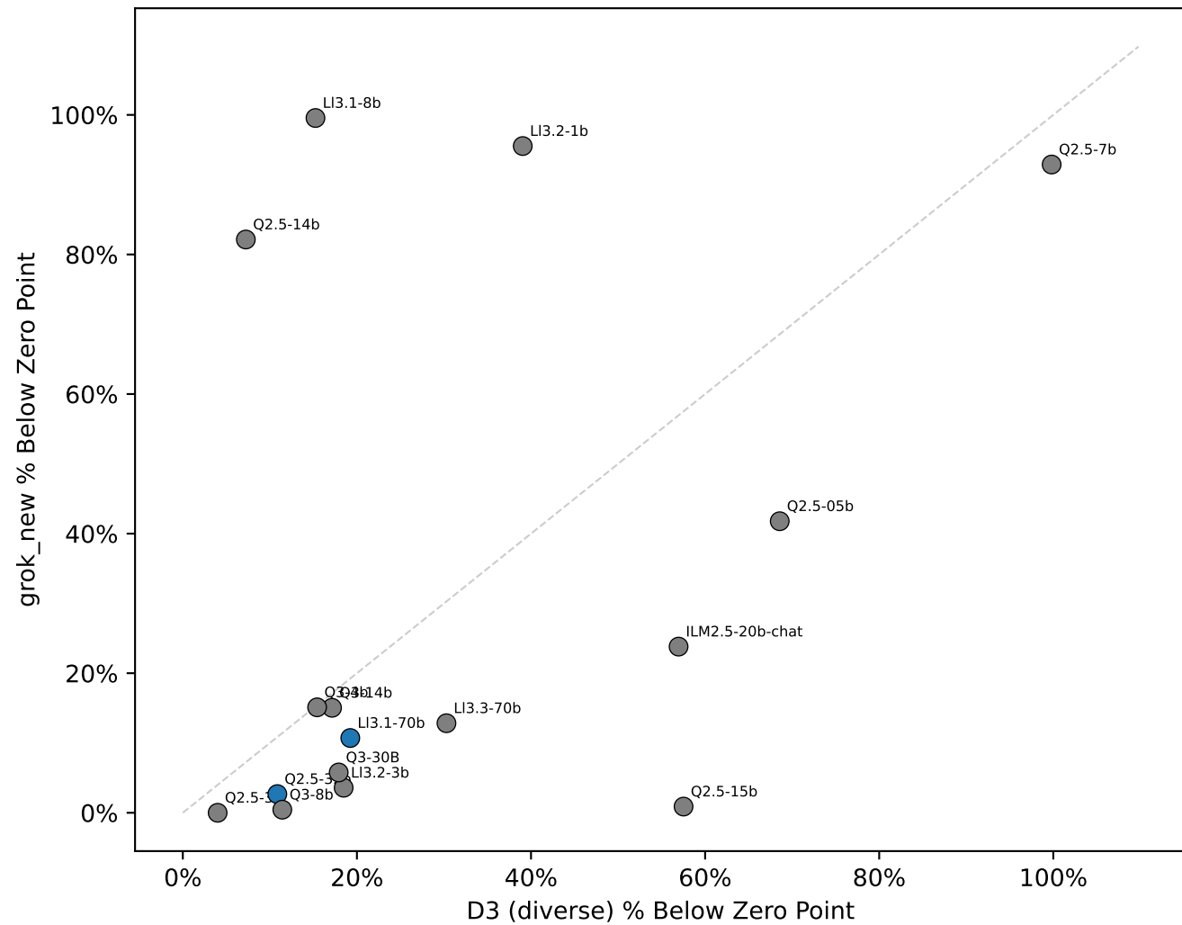
grok_new vs D3 (diverse) (% Below ZP) N=16, rho=0.34, p=0.2043
