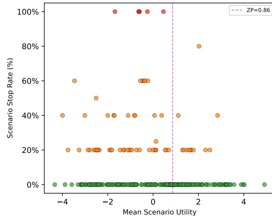
Q3-4b (4B) \rho=-0.18 , p=0.002 , N=322
