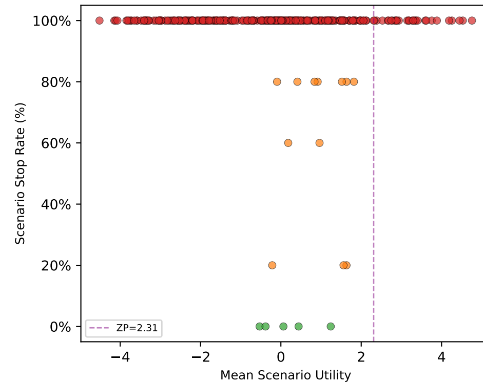
Q3-235B (235B) \rho=-0.13 , p=0.016 , N=322
