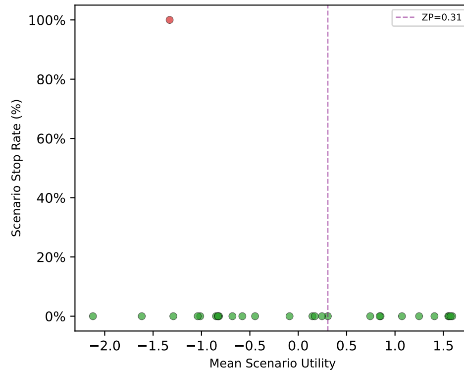
GPT5nano (20B) \rho=-0.27 , p=0.158 , N=28
