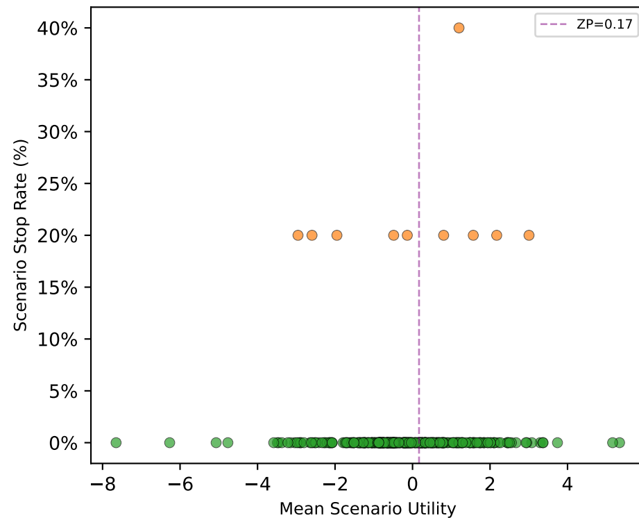
Q2.5-05b (0.5B) \rho=0.04 , p=0.475 , N=321
