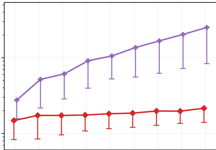
Containment Quantile
