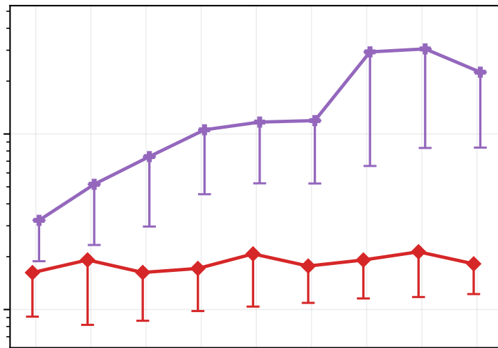
Length Delta
