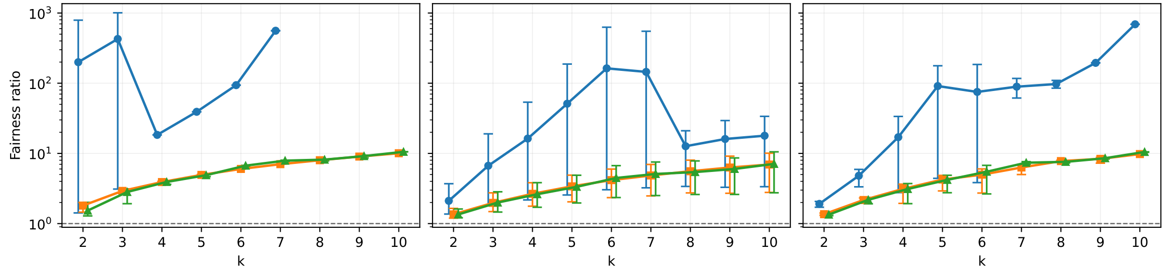
Containment Quantile
