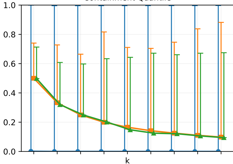
Exponential
