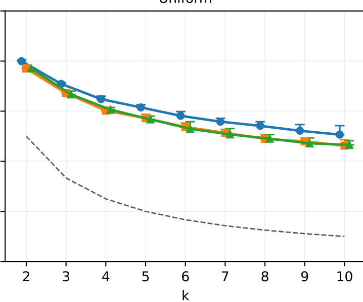
Uniform
