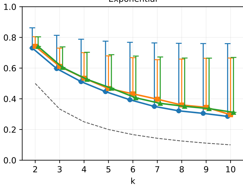
Exponential
