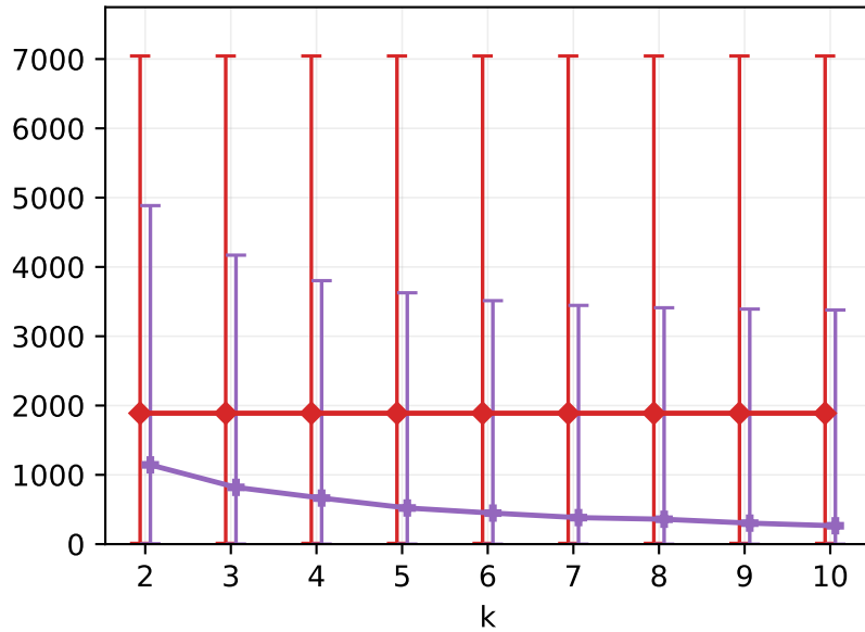
Exponential
