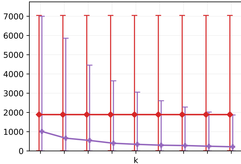
Exponential
