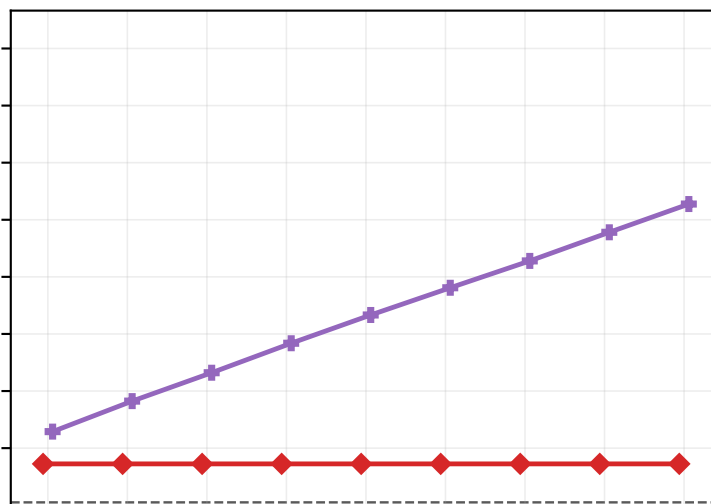
Uniform
