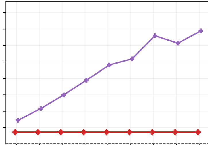
Length Delta
