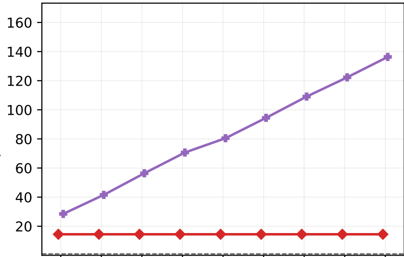
Containment Quantile
