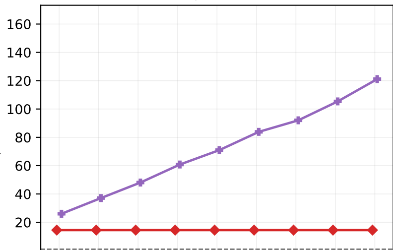
Exponential
