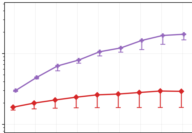
Exponential
