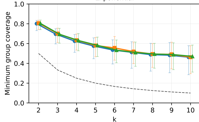
Exponential
