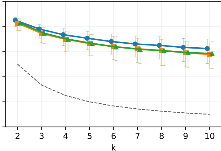
Uniform
