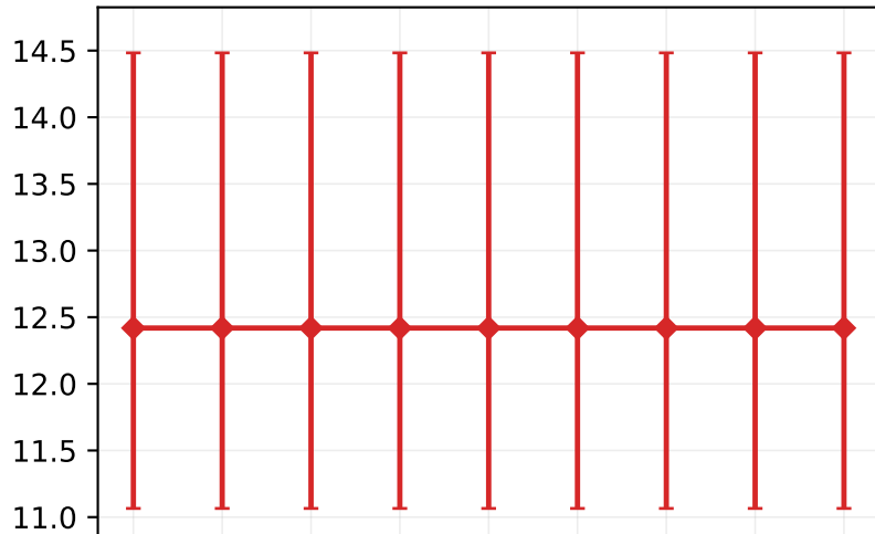
Exponential
