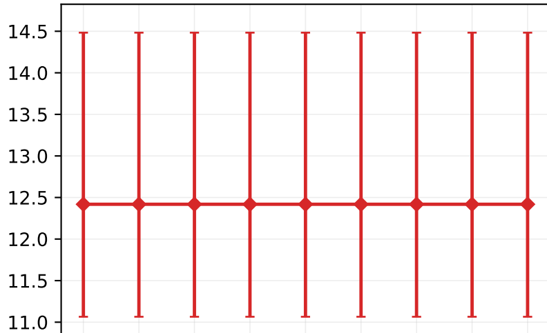
Containment Quantile
