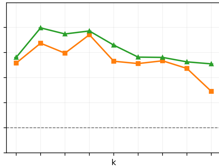
Length Delta
