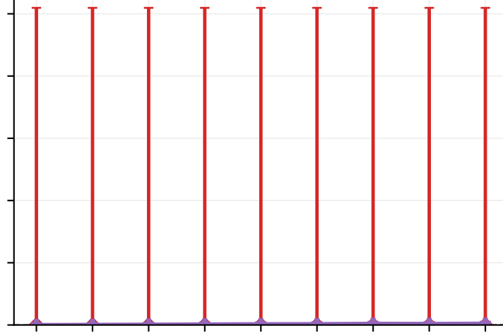
Length Delta
