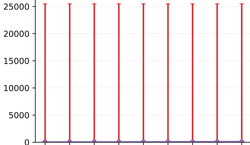
Exponential
