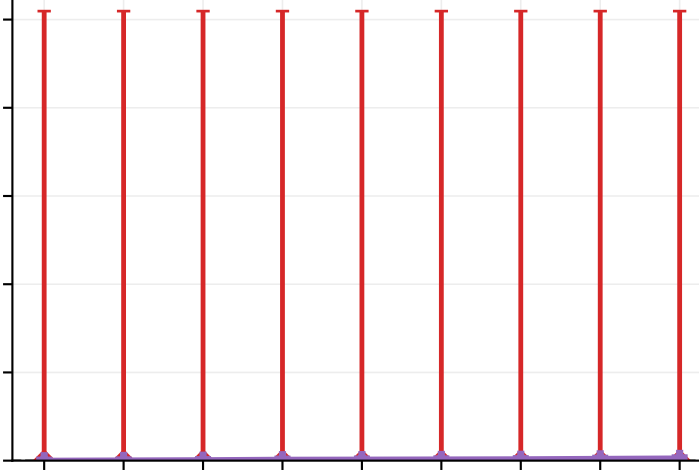
Uniform
