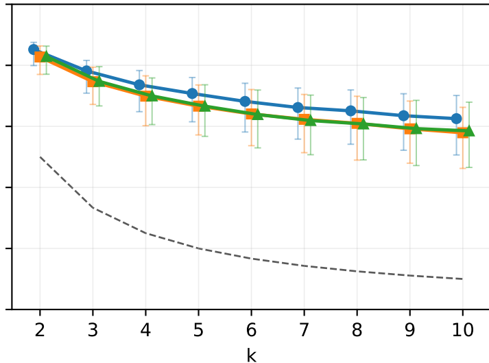
Uniform
