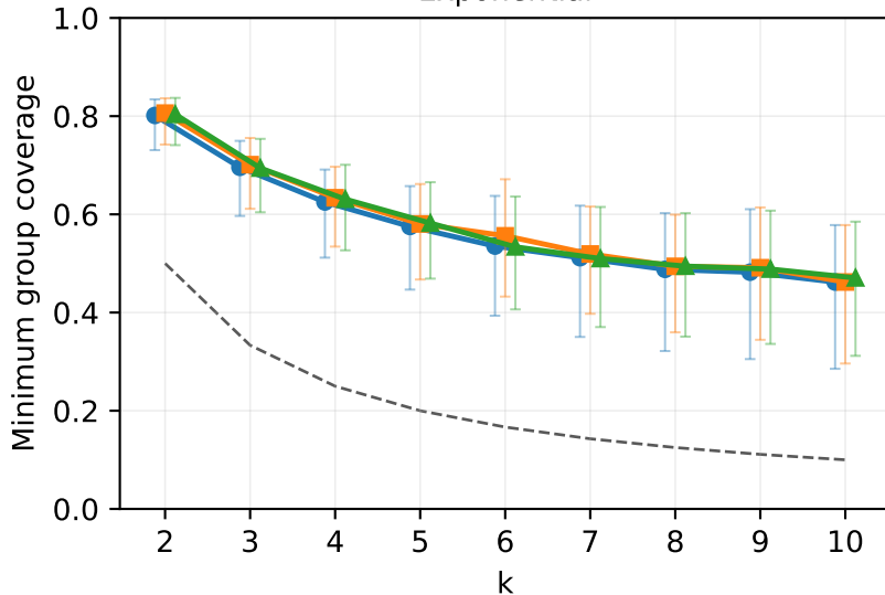
Exponential
