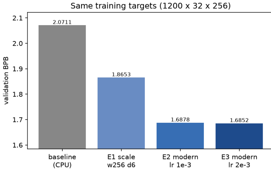
Figure 1: validation BPB at the baseline's training budget (baseline, E1, E2, E3).
