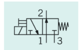
3/2 NO
