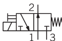
3/2.N.O. (常开触点) (Normally open)
