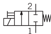
2/2.N.C. (常闭触点) (Normally closed)
