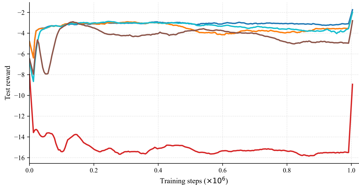
Reward curves
