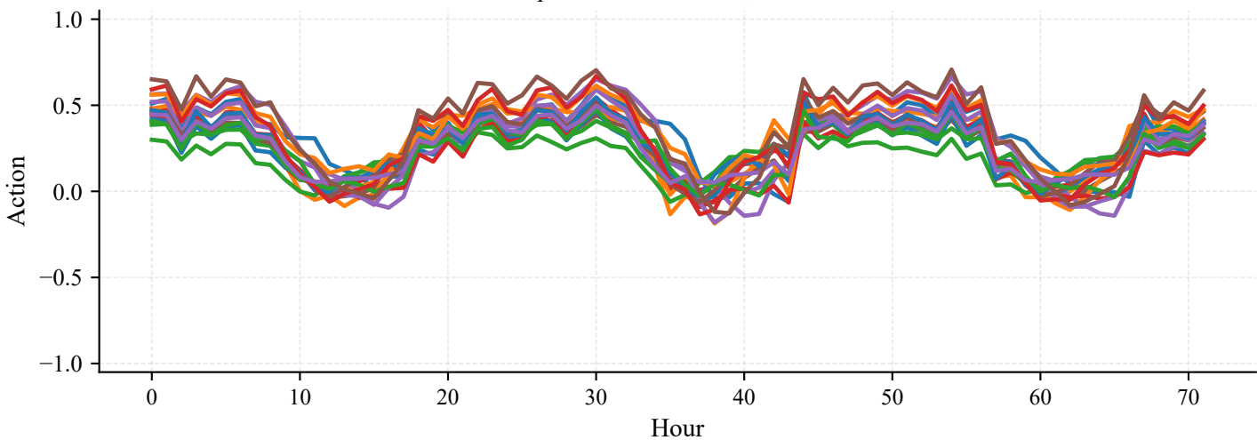
Diffusion-MLP: mean pairwise corr. = 0.880, mean cross-zone std. = 0.082
