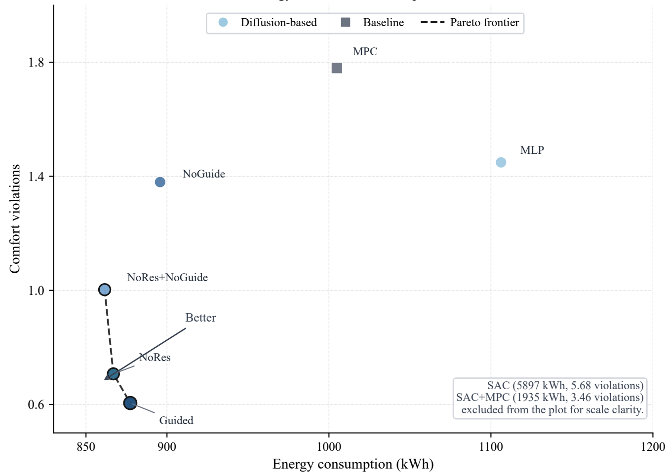
Energy-comfort Pareto comparison
