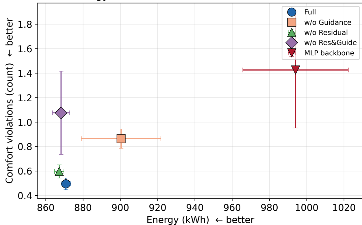
Energy-Comfort Trade-off (OfficeSmall, 3-seed)
