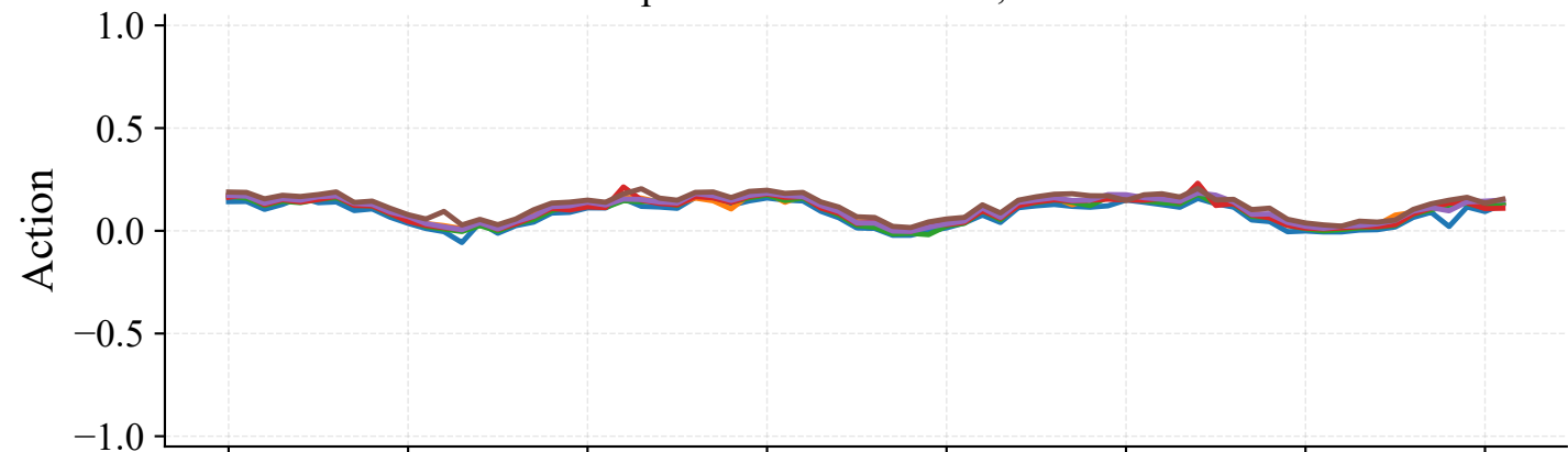
DiffFNO w/o Guidance: mean pairwise corr. = 0.905, mean cross-zone std. = 0.032
