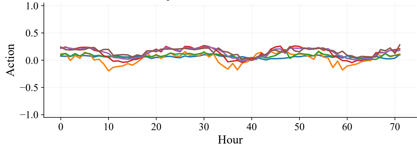
Diffusion-MLP: mean pairwise corr. = 0.560, mean cross-zone std. = 0.061
