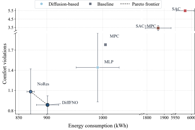
Fig. 3: Energy-comfort Pareto comparison for the evaluated controllers. Learning-based points show three-seed means and error bars show one standard deviation, while MPC is included as a physical reference controller.
