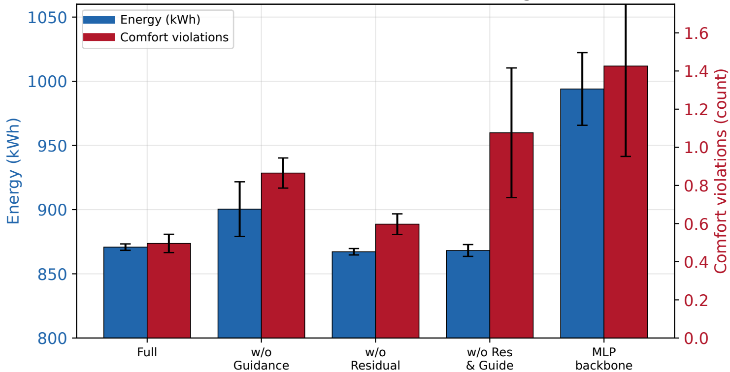
Ablation (OfficeSmall, 3-seed): residual NOT essential; guidance cuts violations
