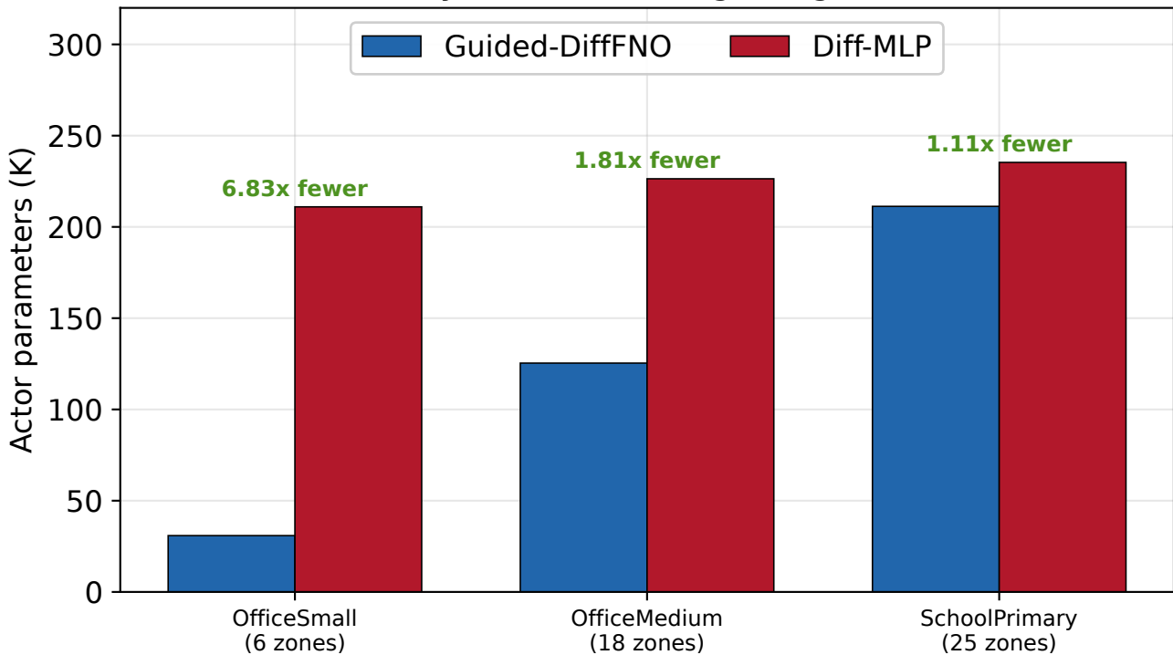
Parameter efficiency: FNO advantage largest on small building
