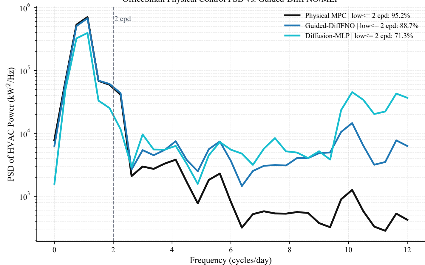
OfficeSmall Physical Control PSD vs. Guided-DiffFNO/MLP
