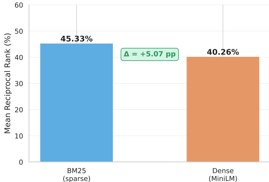
(b) MRR: BM25 outperforms Dense
