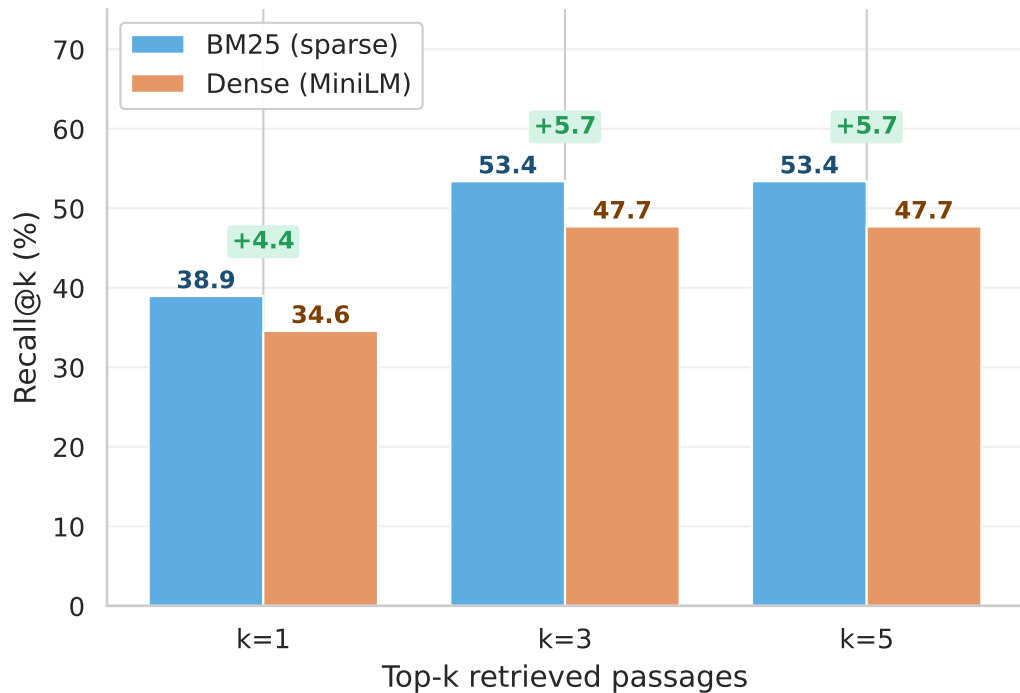
(a) Recall@k: BM25 vs Dense
