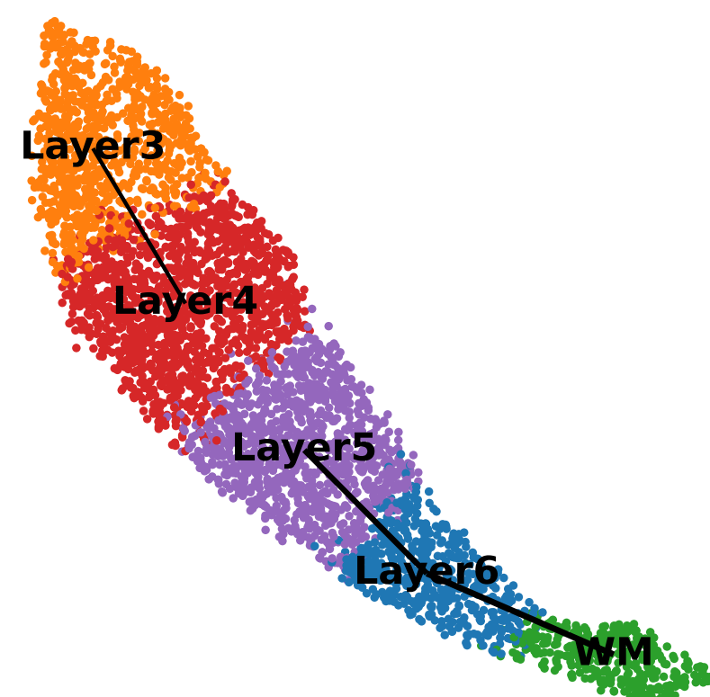
MuCoST
