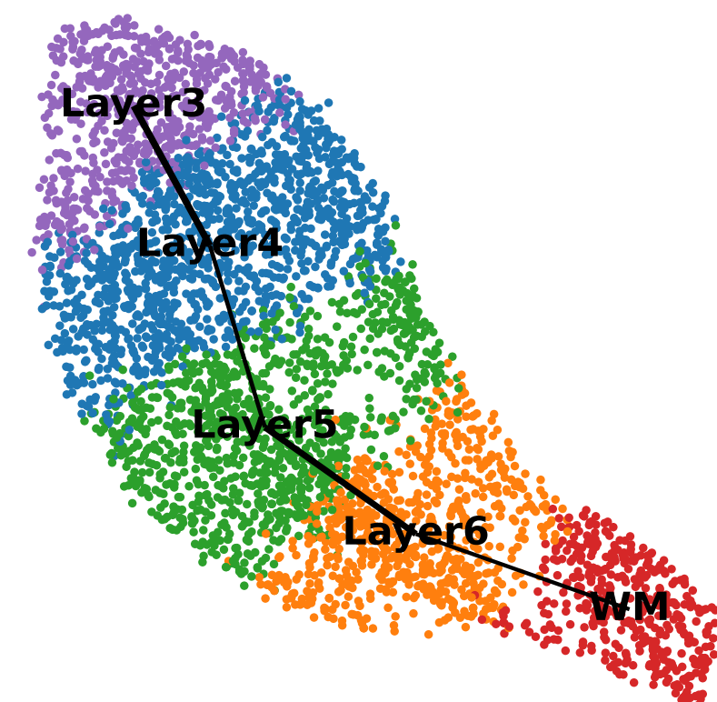
MuCoST
