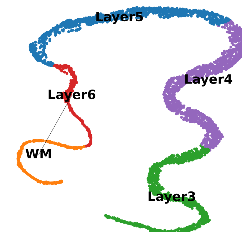
SpaceFlow
