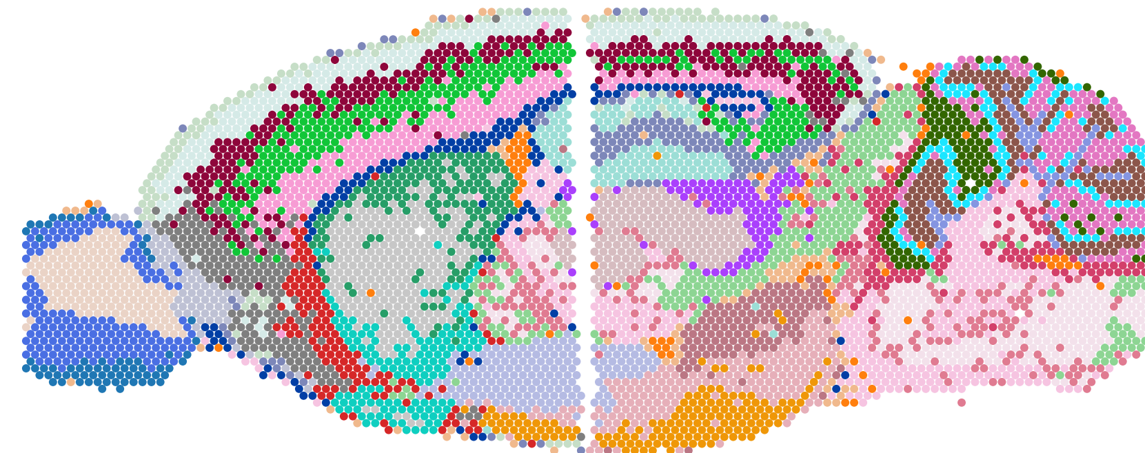
MuCoST
