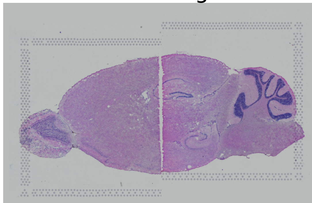
SpaceFlow
