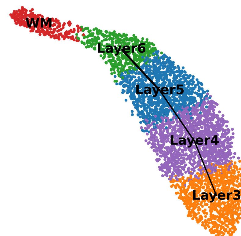
GraphST
