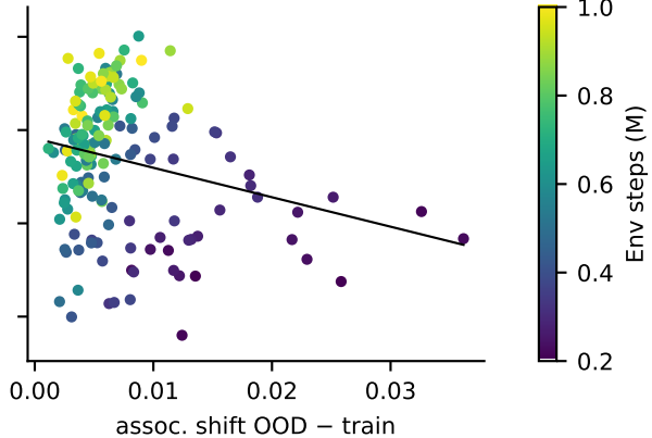
DistractingCS (easy) ( r = -0.24 , n = 162 )
