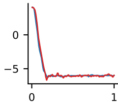
Policy entropy
