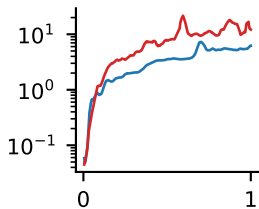
Critic loss
