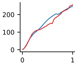
Mean Q
