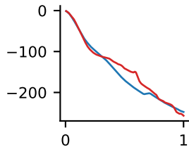
Actor loss
