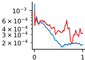
Commitment loss
