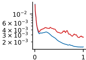
Reconstruction loss
