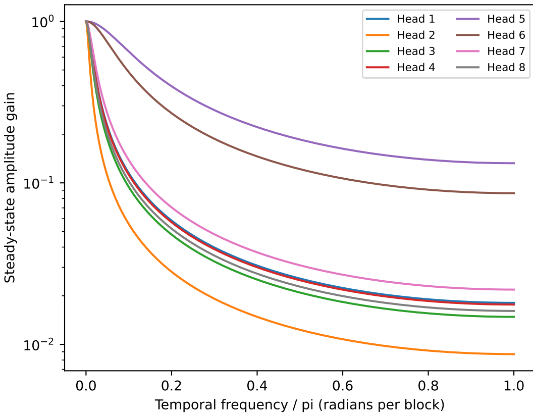
Actual time filter: W's learned EMA
