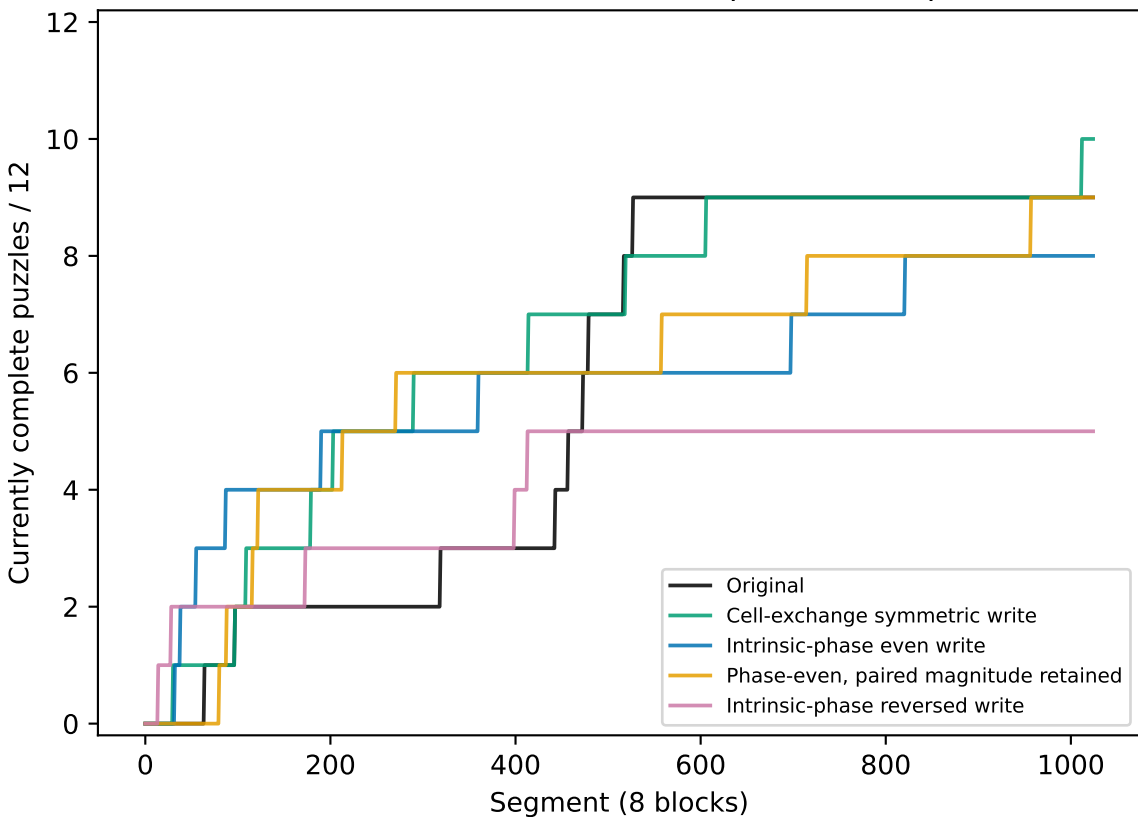
Fresh-state interventions; twelve preselected puzzles
