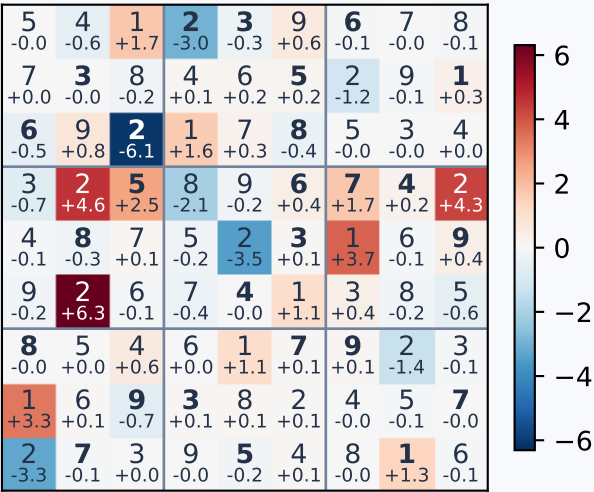
All-head messages to r4c2 Digit 1 minus 2; each tile = one source
