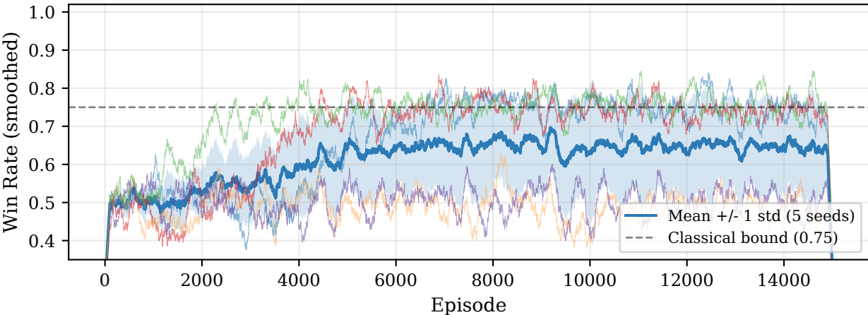
Convergence Across Five Random Seeds
