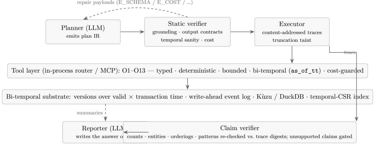
Figure 1: TGMS architecture. The LLM only plans and reports; operators compute; the verifier checks every claim against the execution trace.
